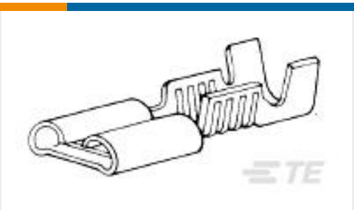
TE Part # 60214-2 187 FASTON REC 20-16 AWG TPBR
