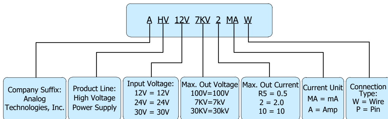
Naming Principle of AHV12V7KV2MAW
