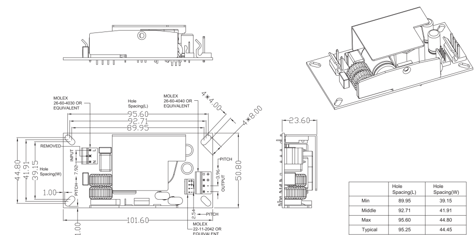
Drawing for the Low Voltage (Range 5-14V):
