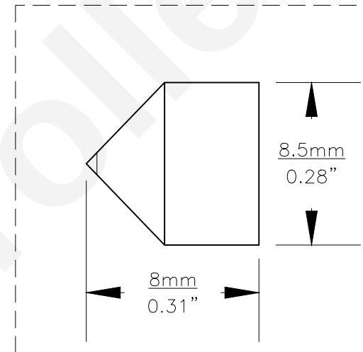
BASE DIMENSIONS
