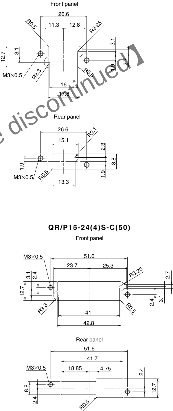
QR/P15-8S-C(50)
