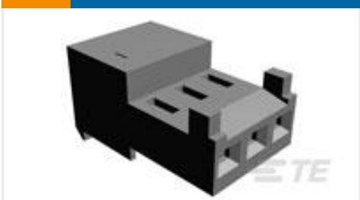
TE Part # 3-644083-3 03P MTA100 CONN ASSY POL TAB
