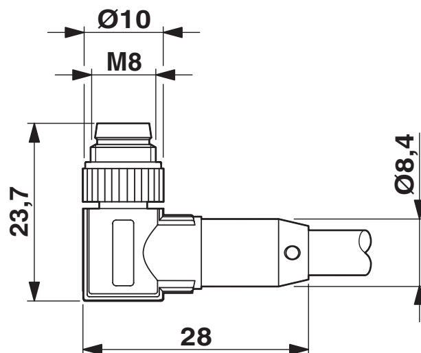
Dimensional drawing
