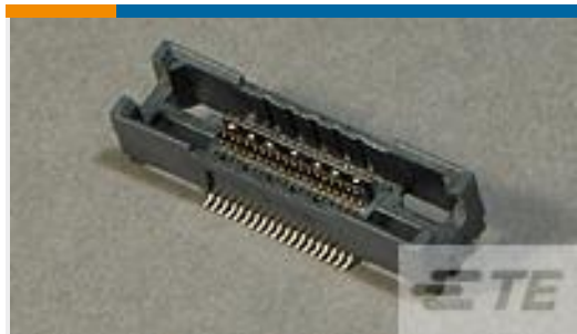
TE Part # 5767054-1 MICT,RECPT,38,ASSY,PDNI
