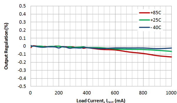
Figure 11. Output Regulation vs. Load Current and Temperature
