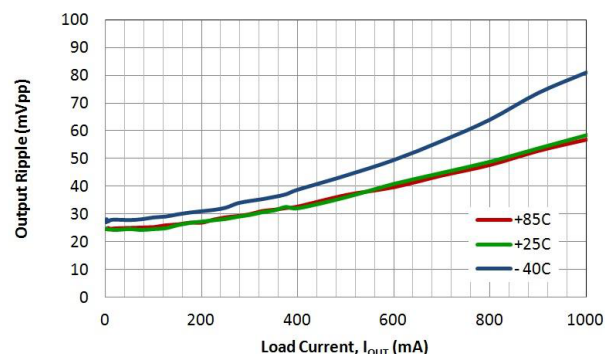
Figure 13. Output Ripple vs. Load Current and Temperature
