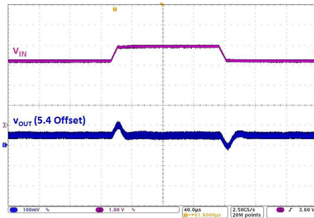
Figure 15. Line Transient, 50 mA, 3.2 V \leftrightarrow 3.9 V, 10 \mu\text{s} Edge
