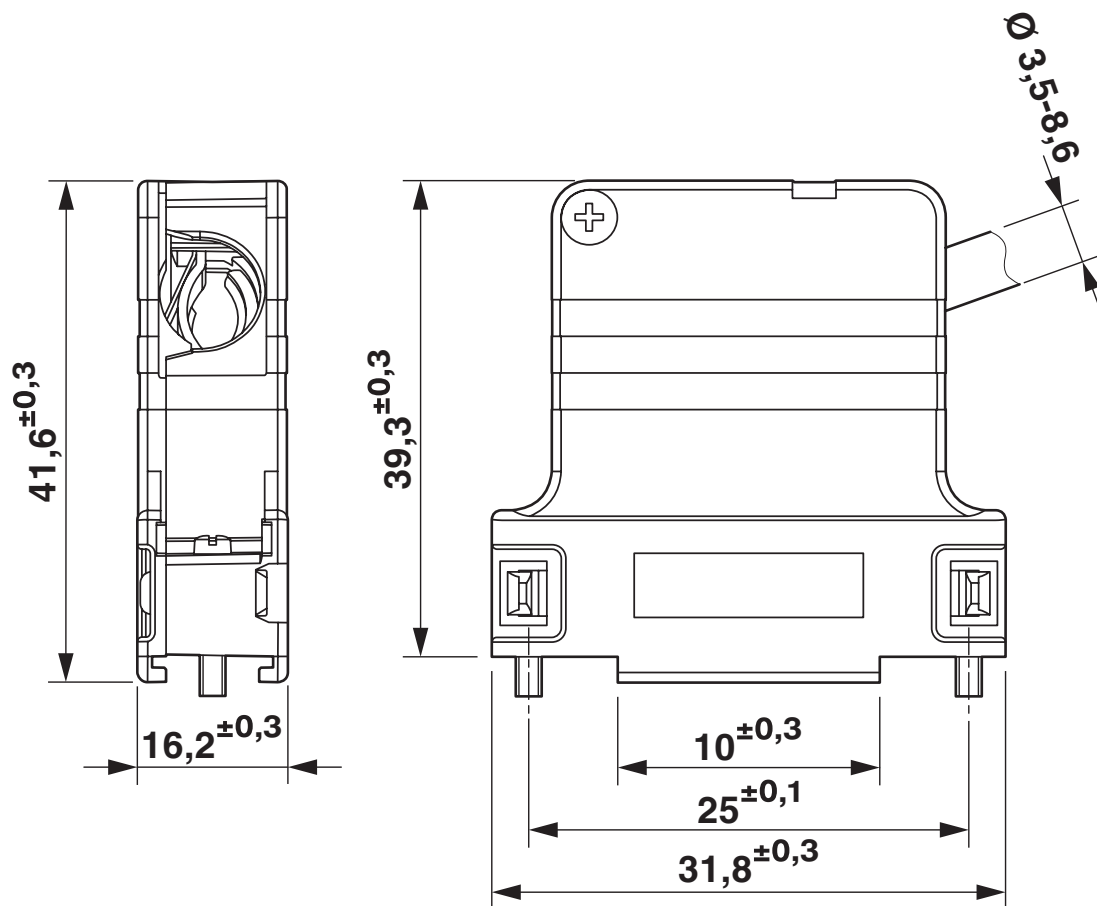
Dimensional drawing
