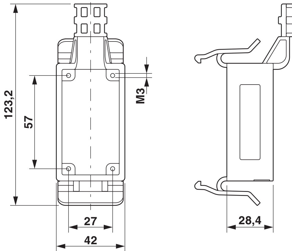
Dimensional drawing
