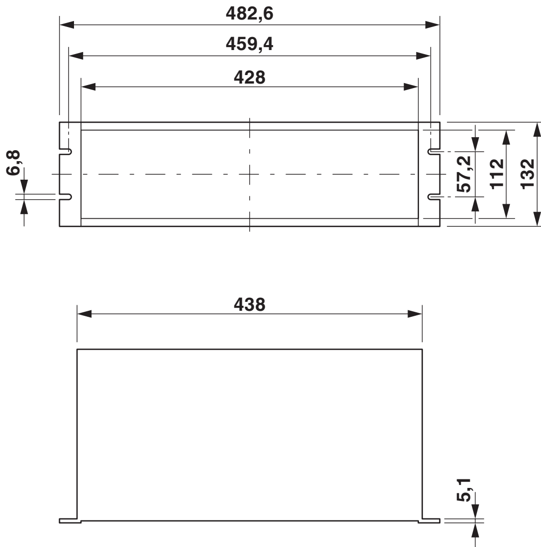
Dimensional drawing
