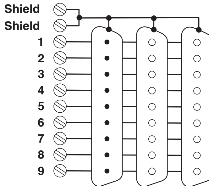
Circuit diagram
