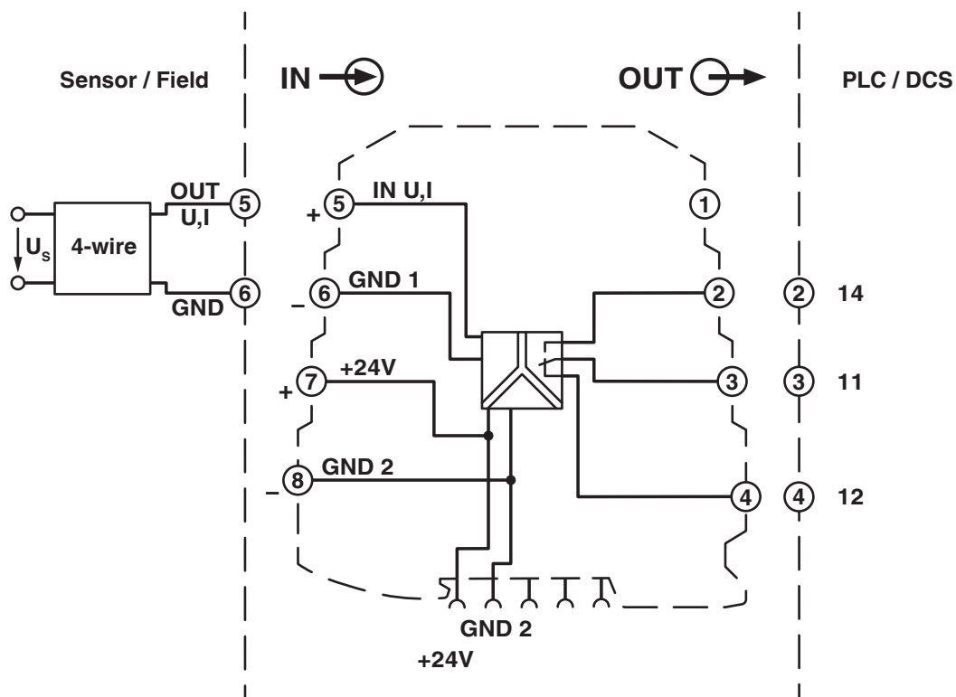
Block diagram
