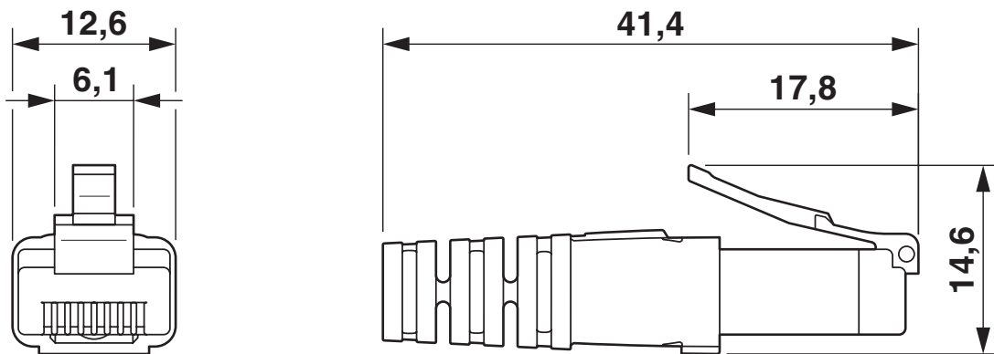
Dimensional drawing
