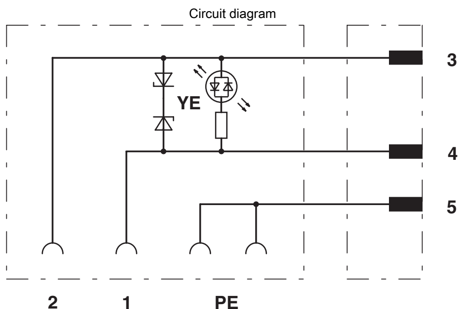
Valve connector, type BI, side view
