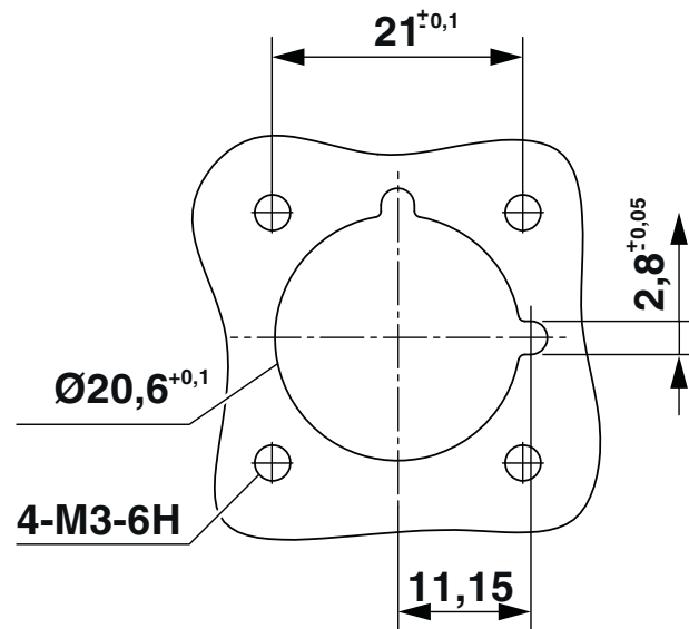
Dimensional drawing
