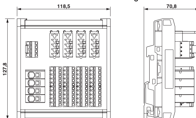
Dimensional drawing
