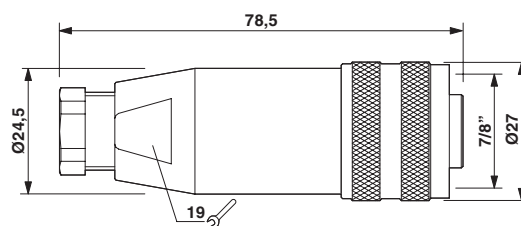
Dimensional drawing
