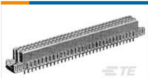
TE Part # 535089-5 096 EURO TYPE C RECEPT ST ASSY
