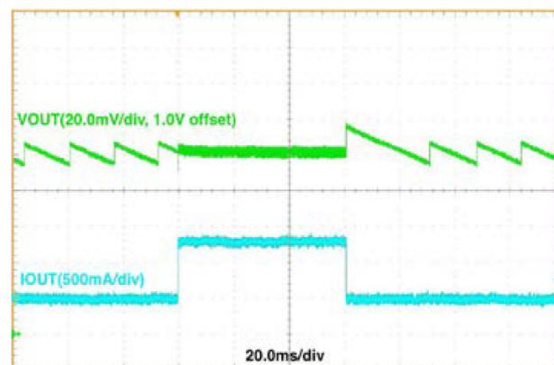
Figure 16. Load Transient, V_{IN} = 3.8\text{ V} , V_{OUT} = 1.125\text{ V} , 0 mA \Leftrightarrow 800 mA, 900 ns Edge, Auto Mode
