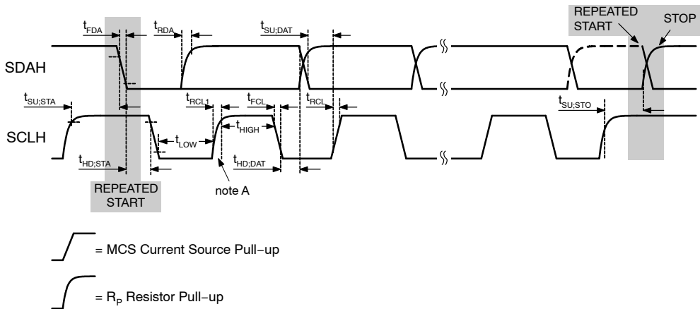
Figure 4. I 2 C Interface Timing for High-Speed Mode
