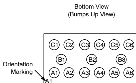
CM1420 CSP Package
