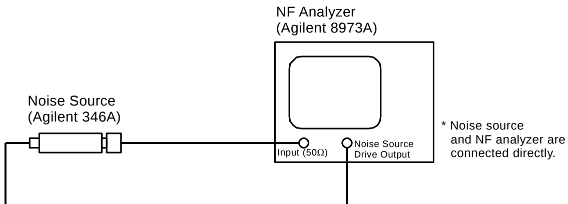
Calibration Setup
