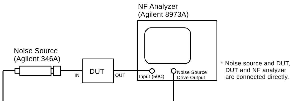
Measurement Setup
