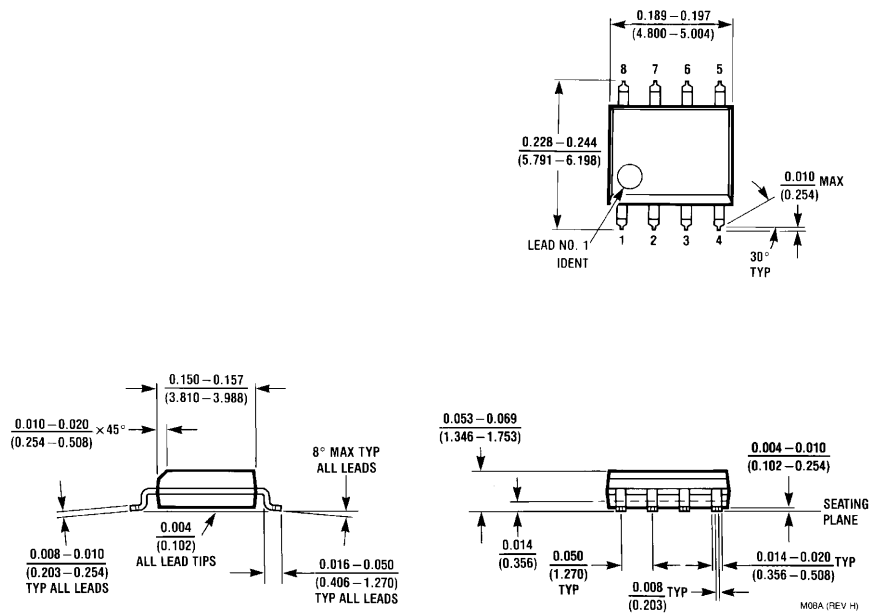
Dual-In-Line Package (M)
