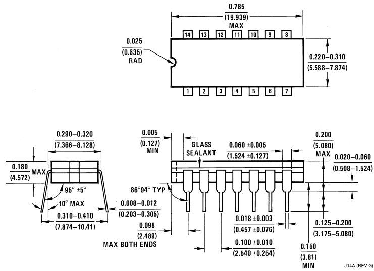
Dual-In-Line Package (J)
