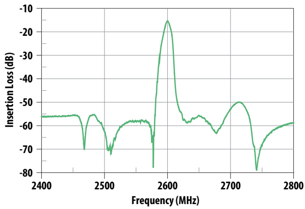
Figure 5. Tx-Rx Isolation.
