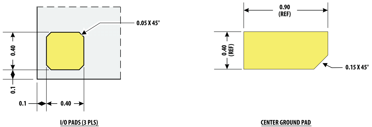
Figure 24. Pad Detail.
