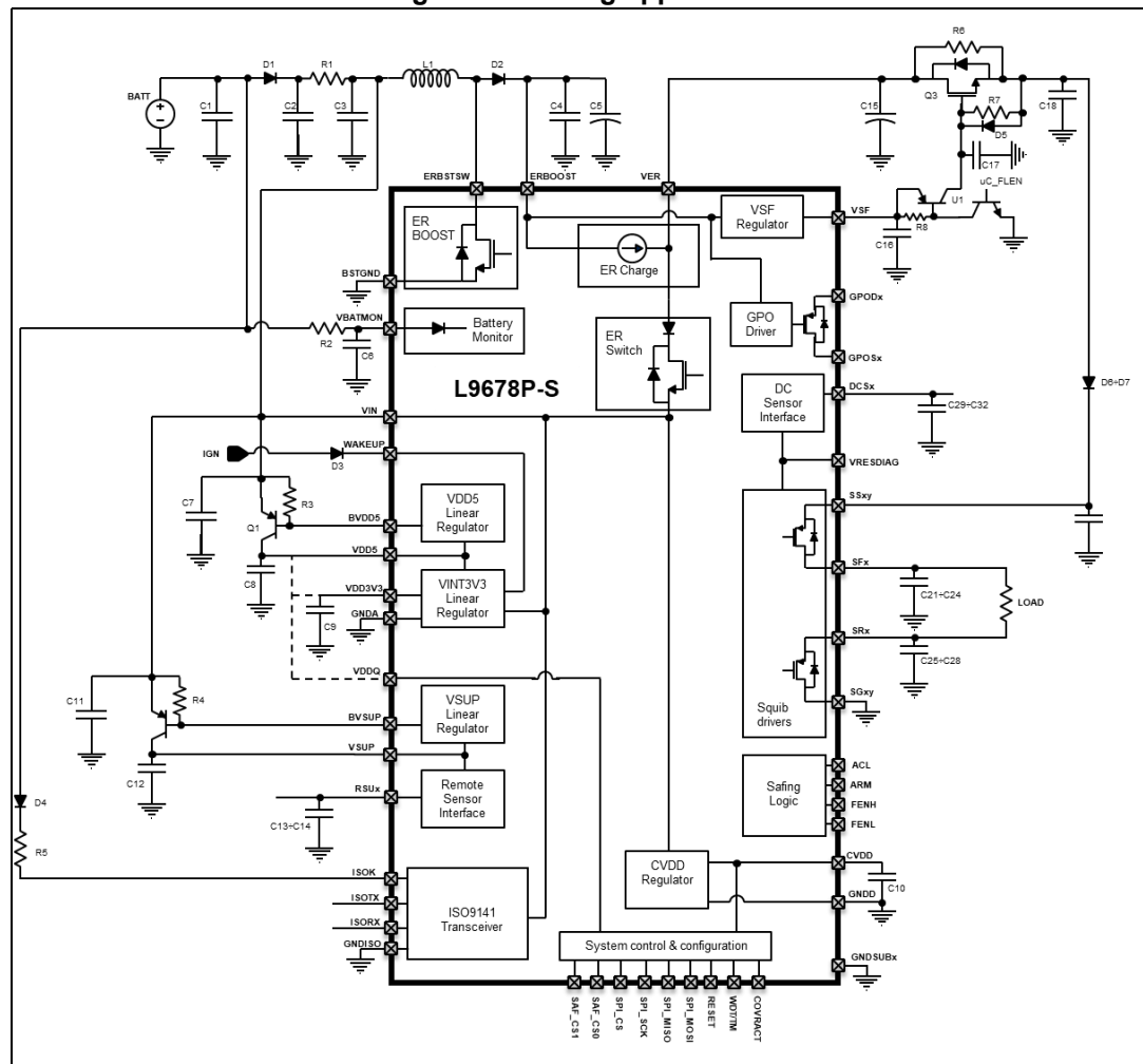
Figure 58. Airbag application
