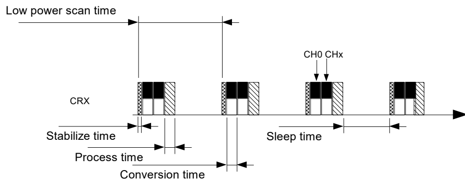
Figure 8.3 Low Power Mode Conversion Process
