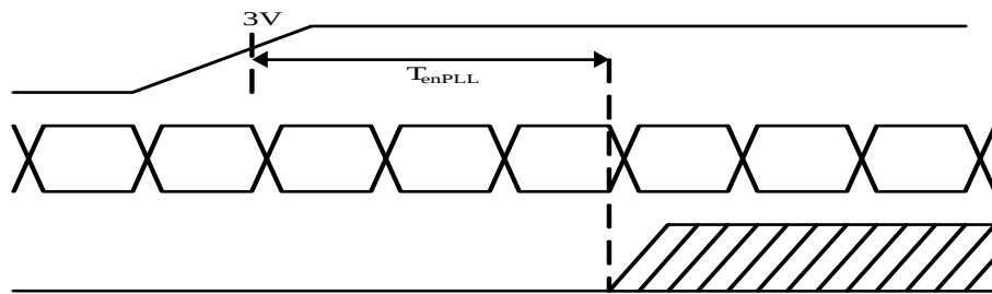
LVDS timing(2)
