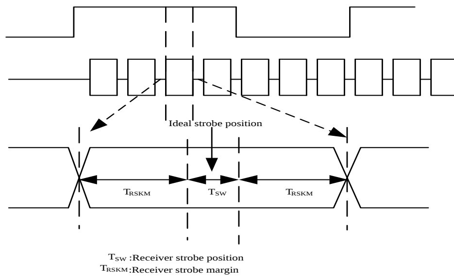
LVDS timing(3)
