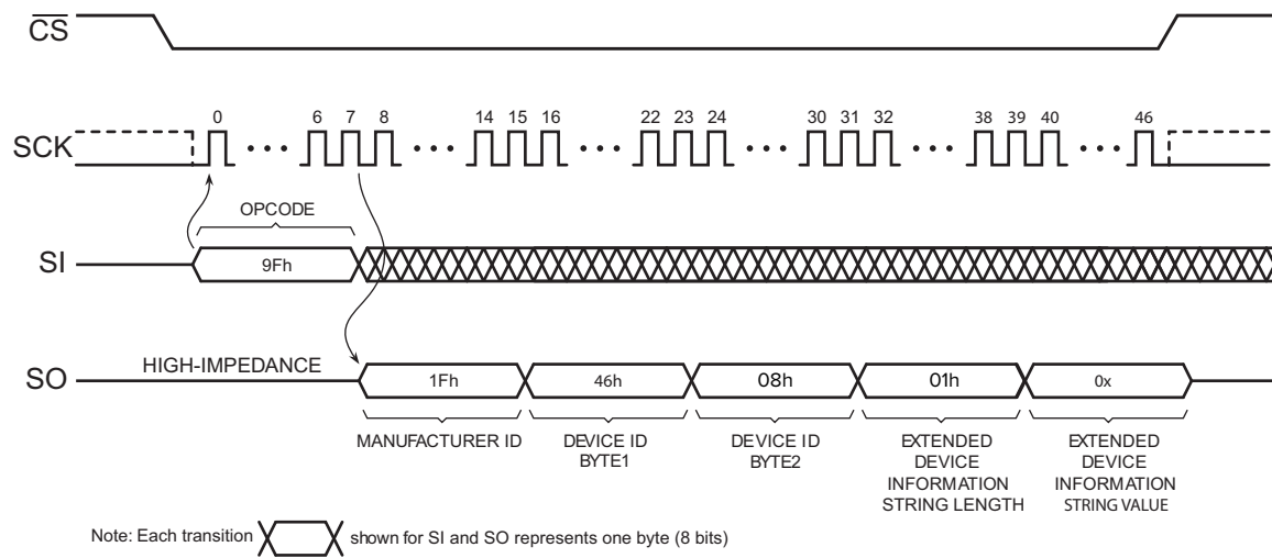
Figure 32: Read JEDEC ID
