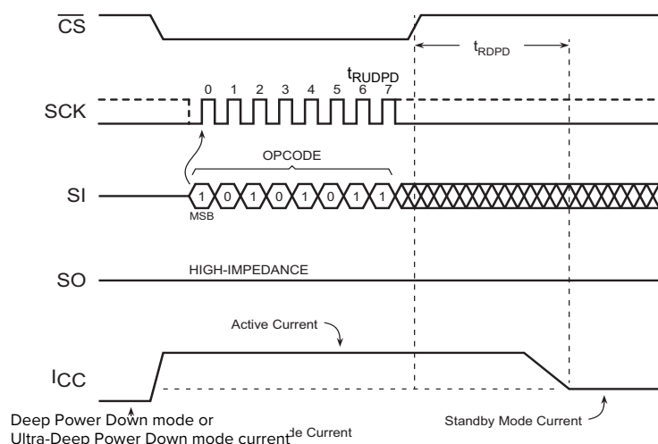
Figure 29: Resume from Deep Power Down or Ultra-Deep Power Down
