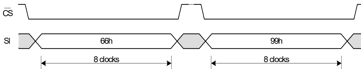
Figure 31: Enable Reset and Reset Command Sequence (SPI Mode)
