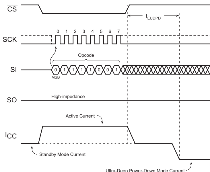
Figure 30: Entering Ultra-Deep Power Down State
