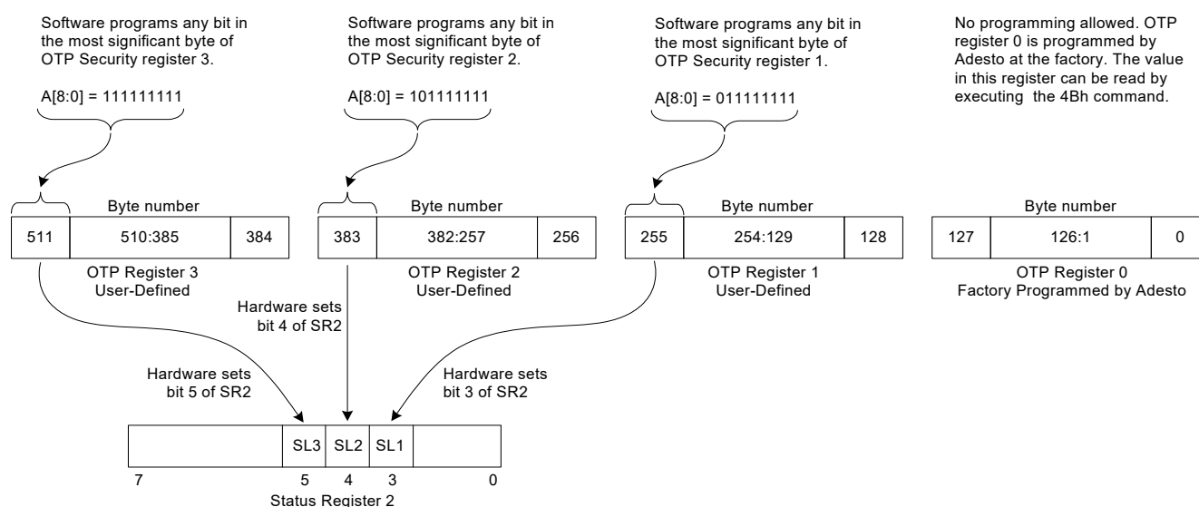
Figure 23: OTP Security Register Program and Lock
