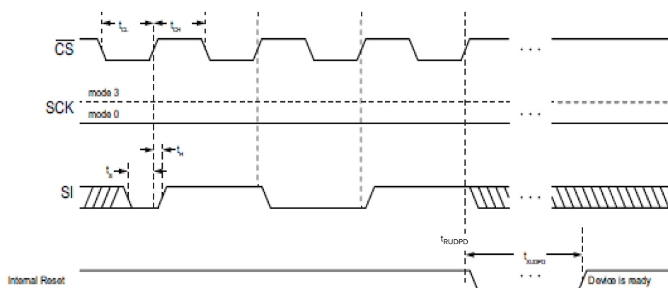
Figure 24: JEDEC Standard Hardware Reset
