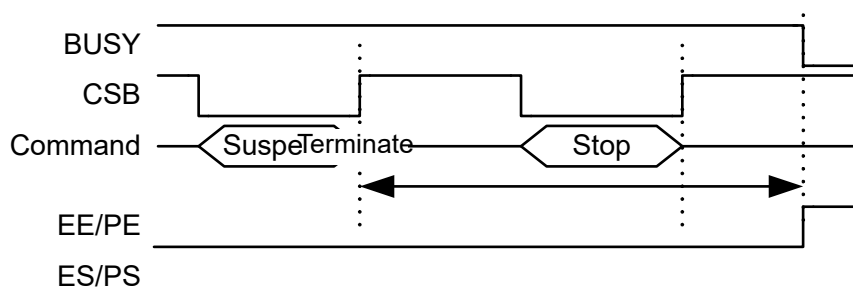
Figure 21: Issuing a Terminate Command Before the Suspend Command has Completed
