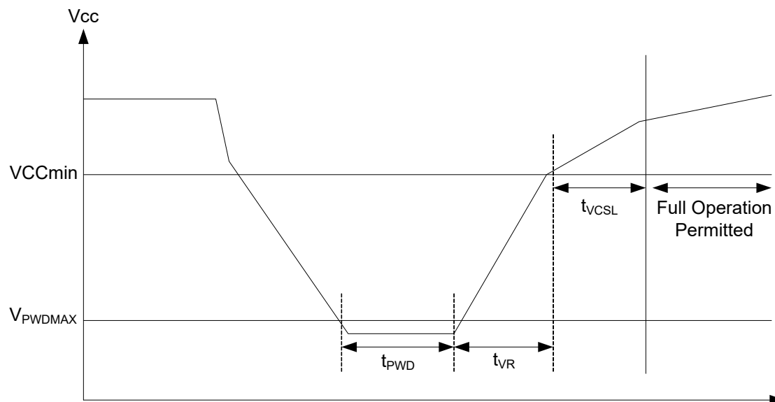
Figure 34: AC Power-up Timing After a Brown-Out
