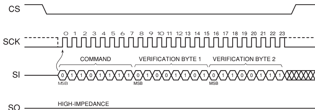
Figure 28: Status Register Lock Operation with Two Verification Bytes
