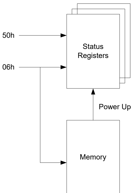
Figure 25: AT25FF161A Register Structure
