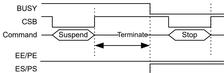
Figure 22: Allowing Enough Time for the Suspend Operation to Complete
