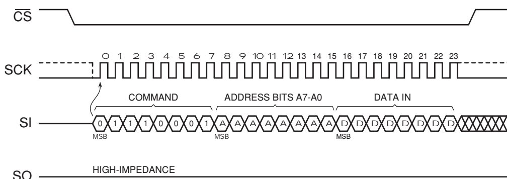
Figure 27: Status Register Write Operation Showing 8-bit Address Field
