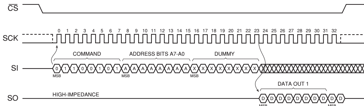
Figure 26: Status Register Read Operation Showing 8-bit Address Field
