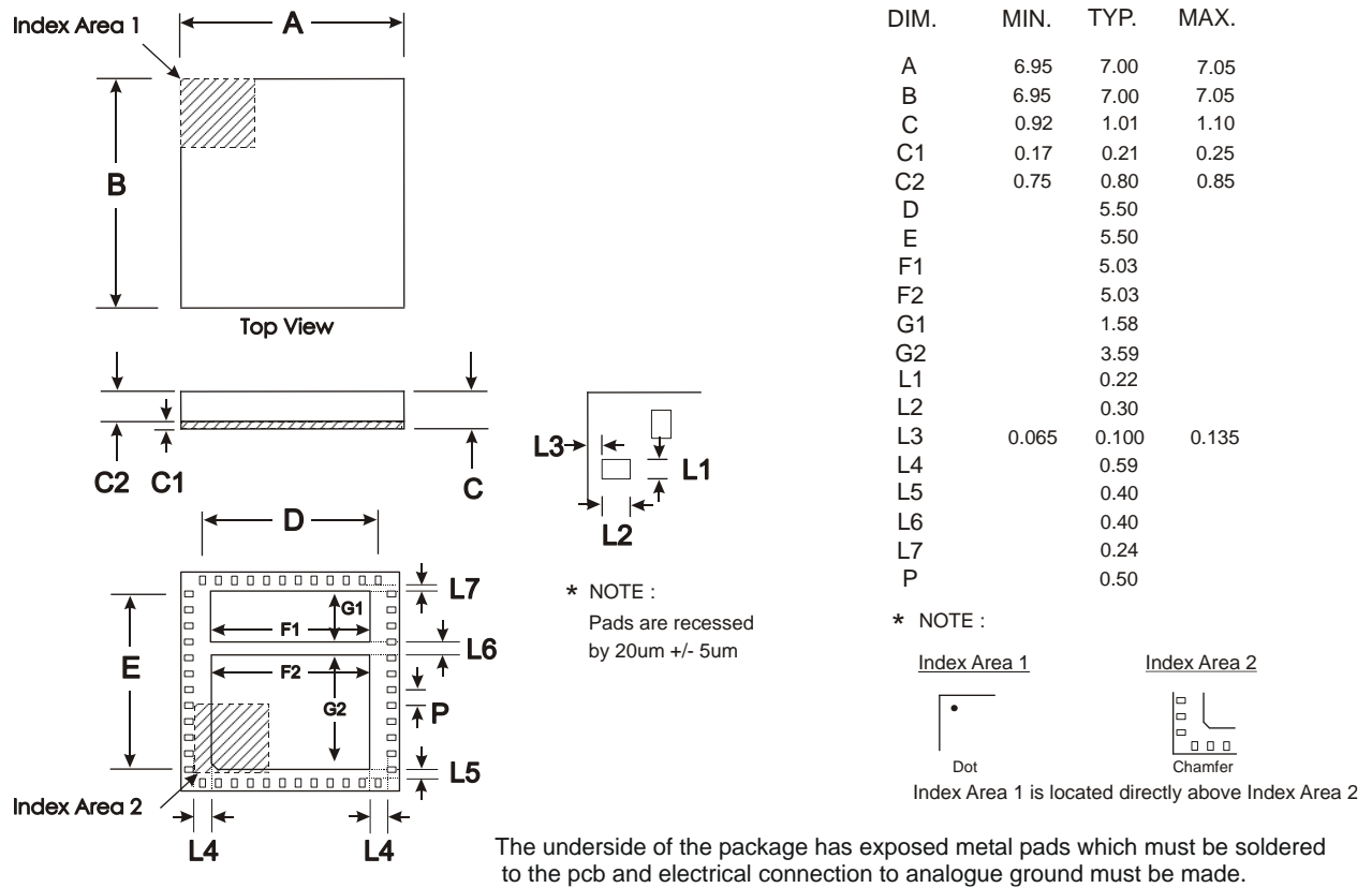
Figure 22 T1 Mechanical Outline
