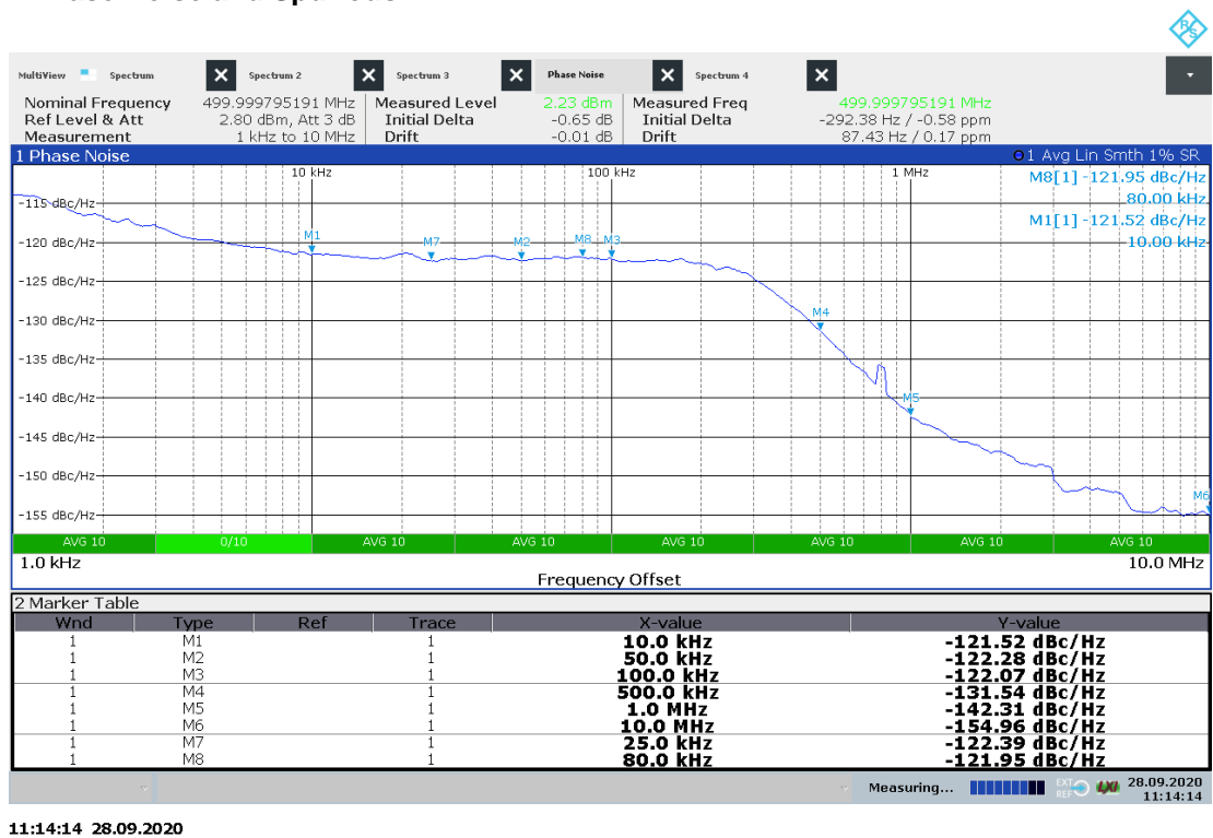
Figure 15 Typical Phase Noise at 500 MHz RF Output
