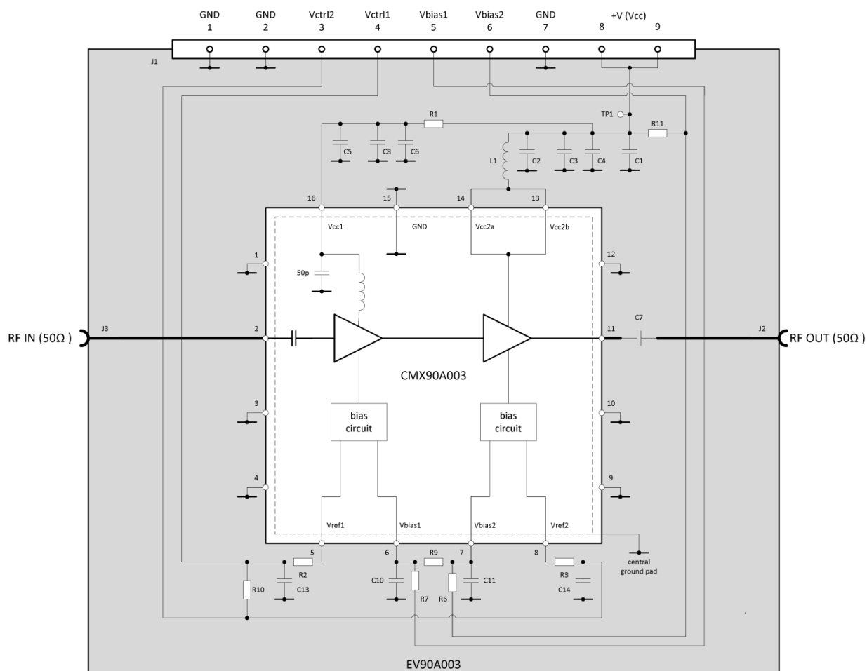
Figure 30: EV90A003 Schematic
