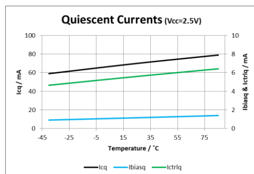
Figure 24: Quiescent Currents
