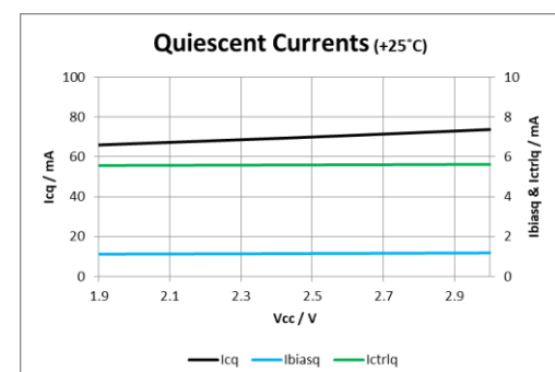
Figure 25: Quiescent Currents
