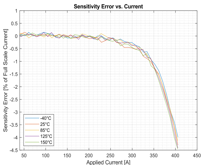
Figure 2: Sensitivity Error in Percent of Full-Scale Current vs. Applied Current
