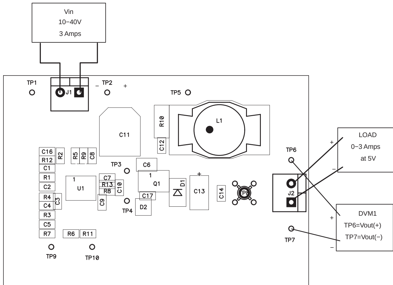
Figure 2. Test Setup
