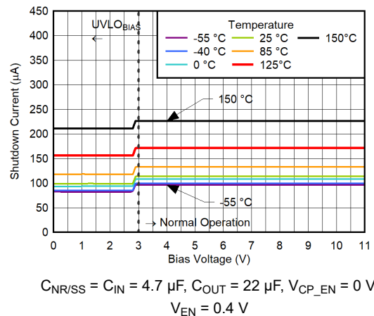
Figure 6-206. IN Pin Shutdown Current vs V_{BIAS} for V_{IN} = 6\text{ V} , V_{OUT(nom)} = 0.5\text{ V} , CP Disabled
