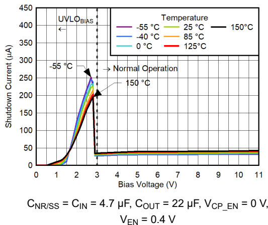
Figure 6-205. BIAS Pin Shutdown Current vs V_{BIAS} for V_{IN} = 6\text{ V} , V_{OUT(nom)} = 0.5\text{ V} , CP Disabled
