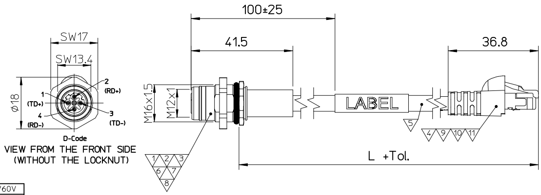
CONNECTOR SPECIFICATION:
