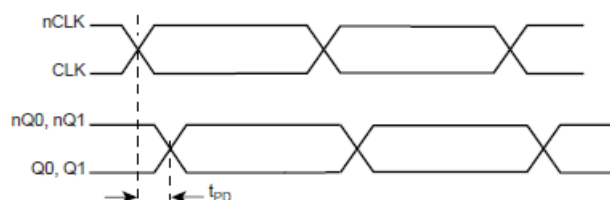
PROPAGATION DELAY
