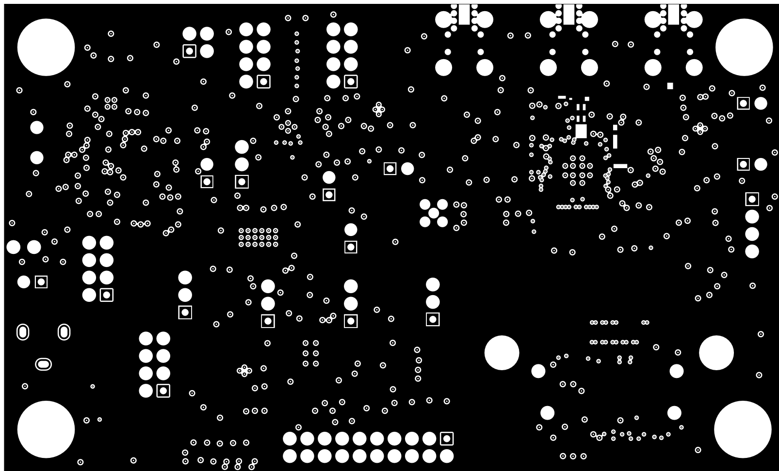
Figure 16-5. Layer 4: GND Plane 2
