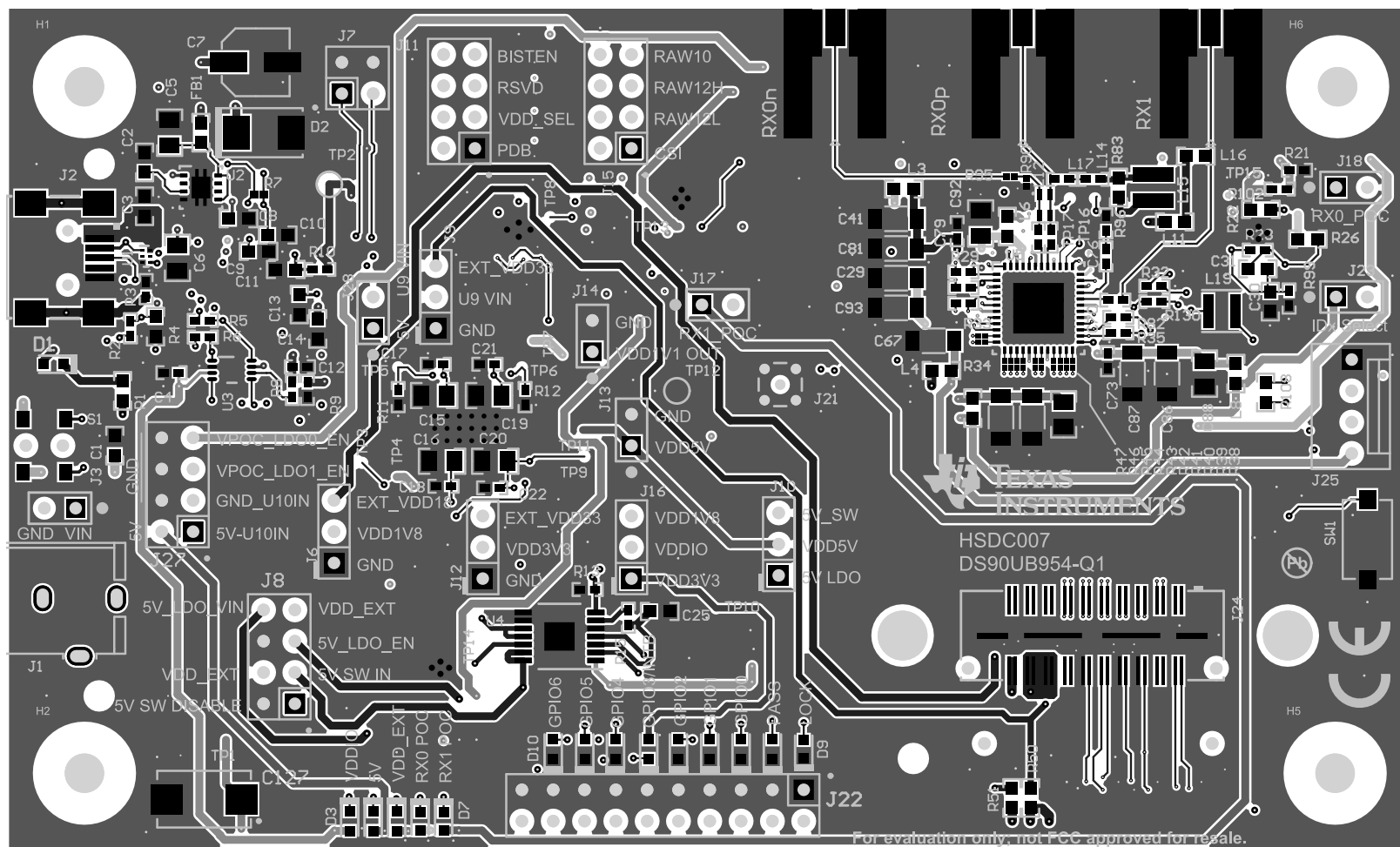
Figure 16-1. Top View Composite
