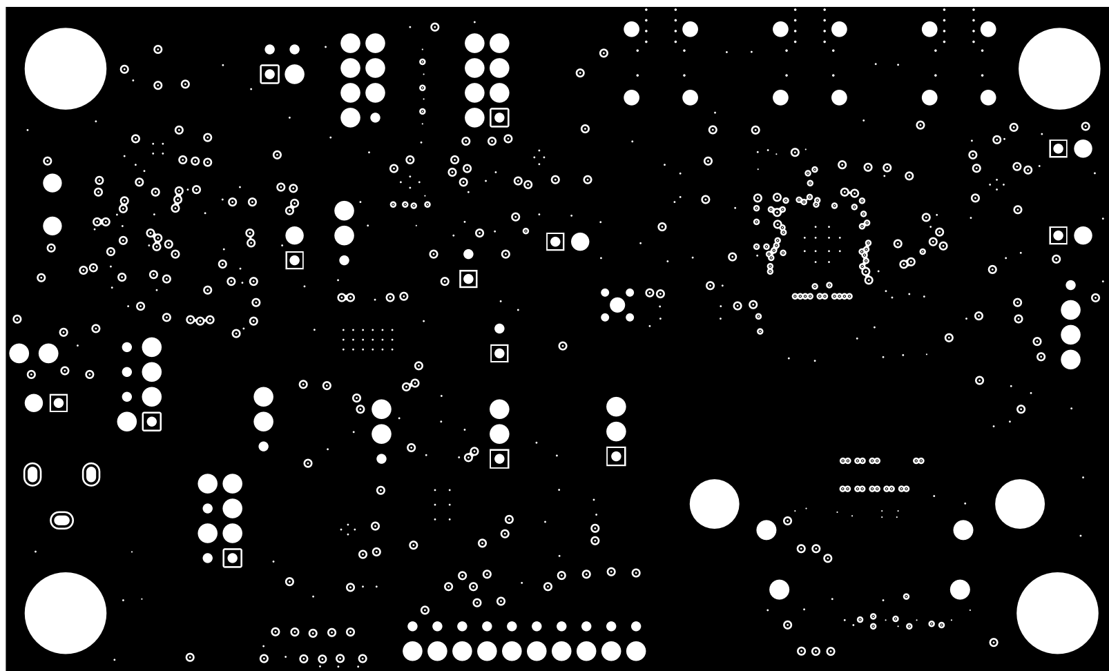
Figure 16-8. Layer 7: GND Plane 4
