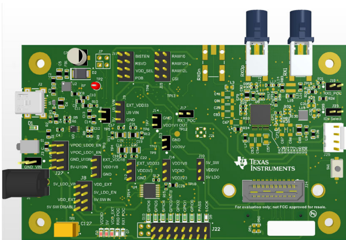
Figure 2-1. DS90UB95x-Q1EVM
