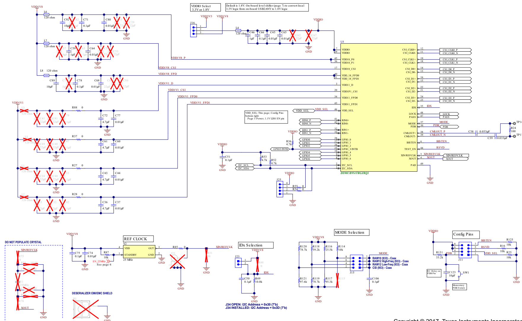
Figure 15-2. DS90UB95x-Q1EVM Main Circuit - Page 1
