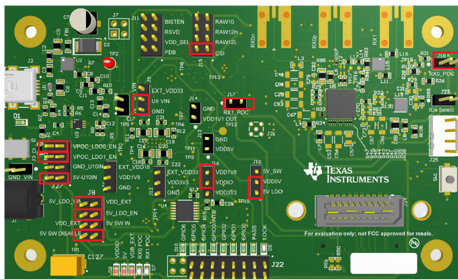
Figure 4-1. DS90UB95x-Q1EVM with Jumpers Highlighted
