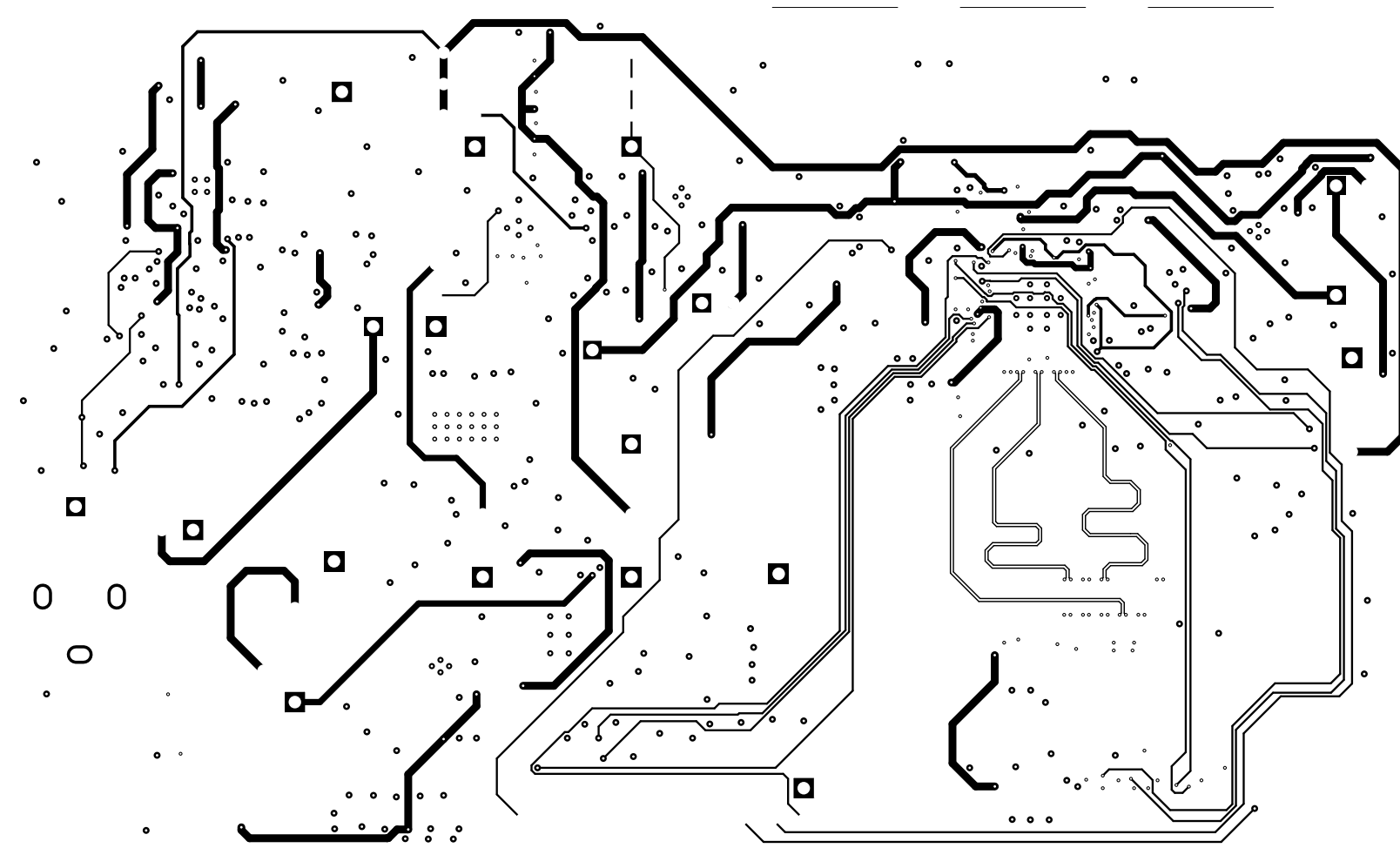
Figure 16-7. Layer 6: Mid Signal Layer 2
