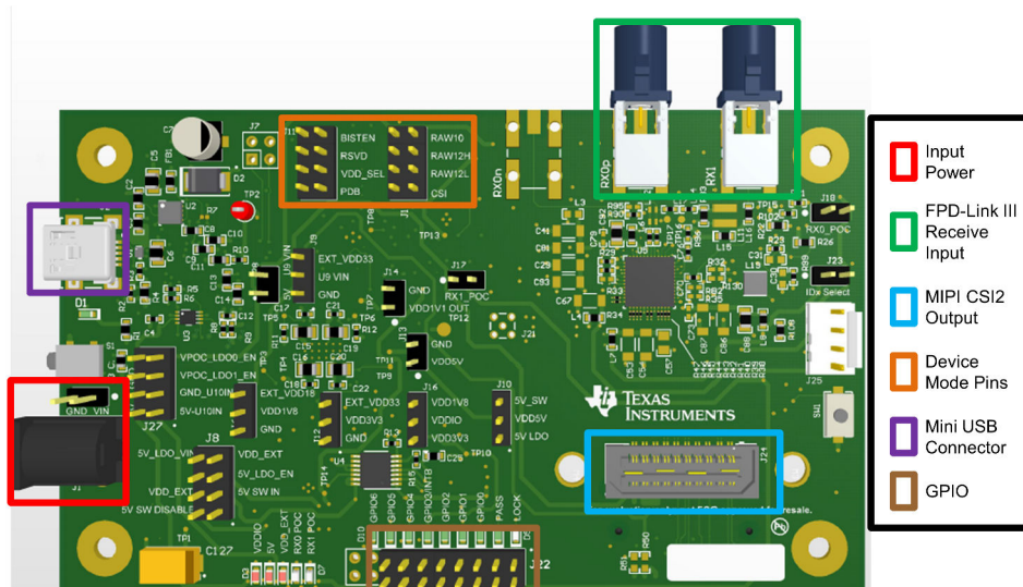
Figure 3-2. Interfacing to the EVM
