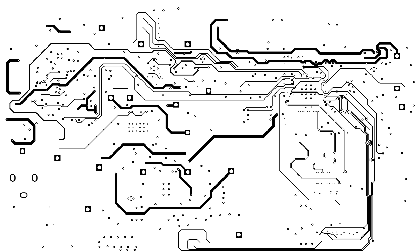
Figure 16-4. Layer 3: Mid Signal Layer 1
