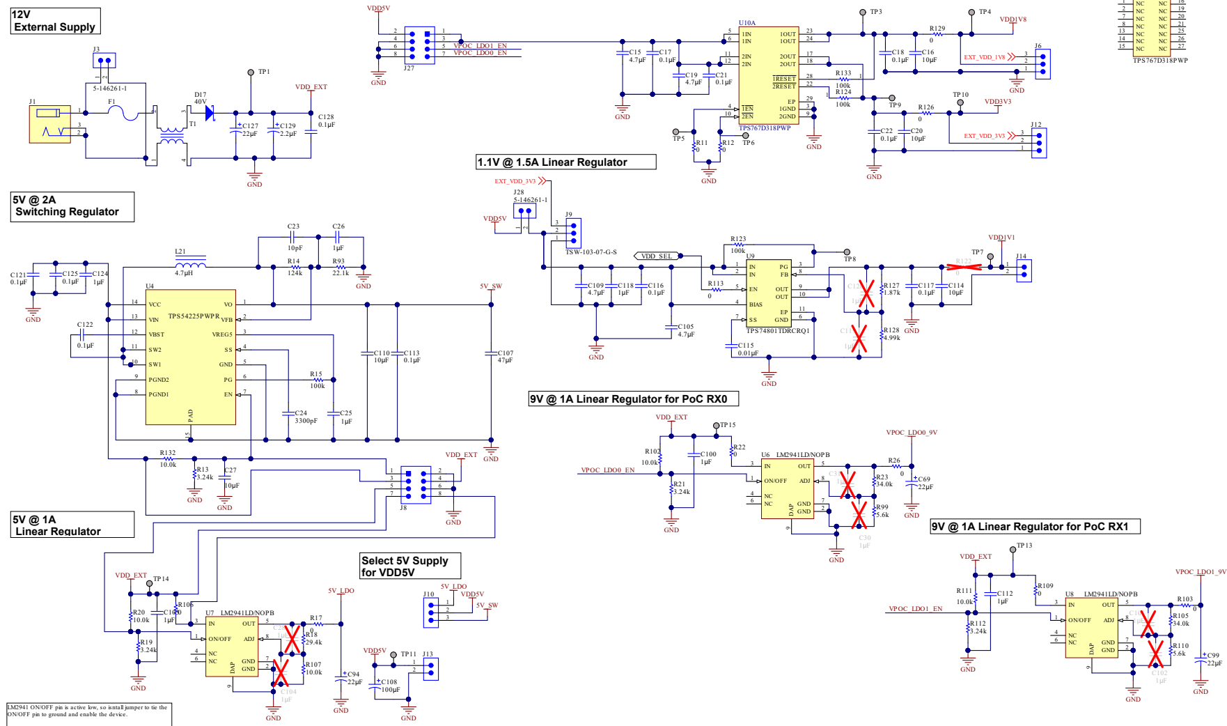
Figure 15-5. DS90UB95x-Q1EVM Power Distribution Circuits - Page 4
