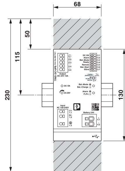
Figure 2 Keep-out areas
