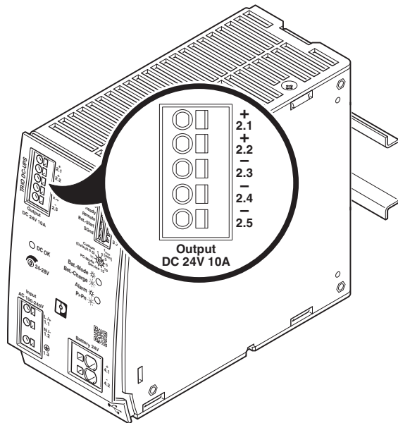
Figure 17 Output voltage connection terminal blocks: Output DC +/-
