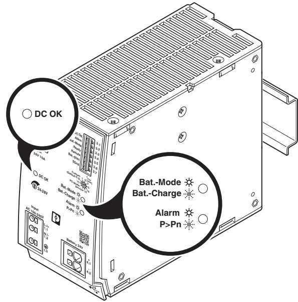
Figure 37 LED indicators
