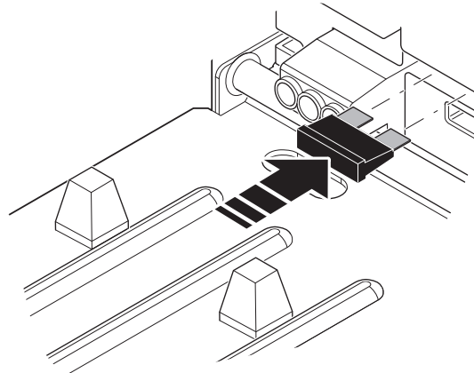
Figure 29 Insert fuse
