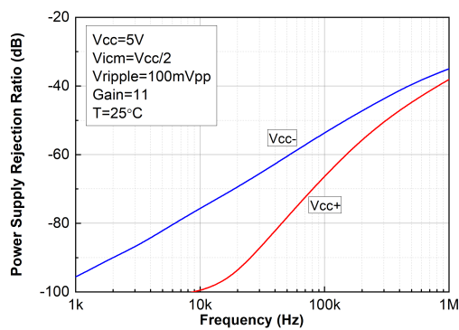
Figure 42. PSRR vs. frequency at V_{CC} = 5\text{ V}
