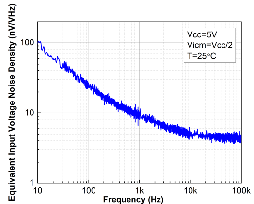
Figure 37. Noise vs. frequency
