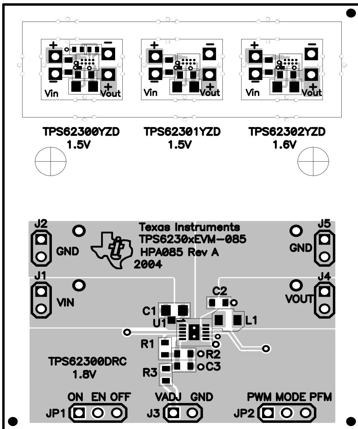
Figure 3. Assembly Layer
