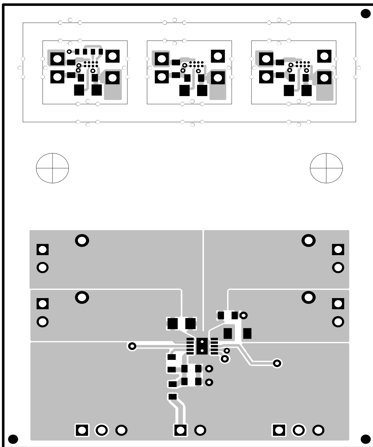
Figure 1. Top Layer Routing
