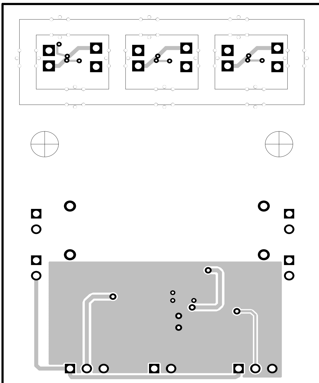
Figure 2. Bottom Layer Routing
