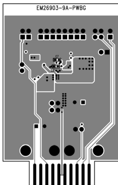
Figure 12. MIC26901 Evaluation Board Bottom Layer
