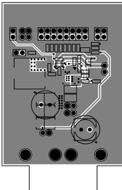
Figure 11. MIC26901 Evaluation Board Mid-Layer 2
