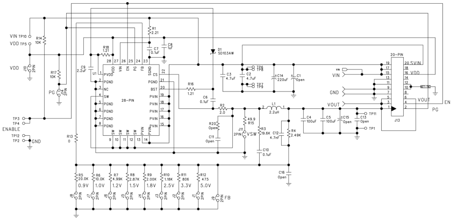
Figure 8. Schematic of MIC26901 Evaluation Board (J11, R13, R15 are for testing purposes)
