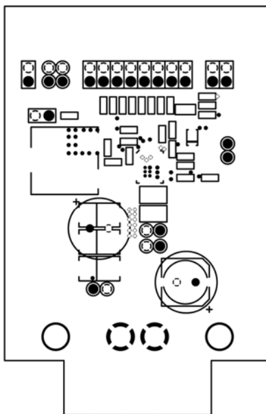
Figure 10. MIC26901 Evaluation Board Mid-Layer 1 (Ground Plane)
