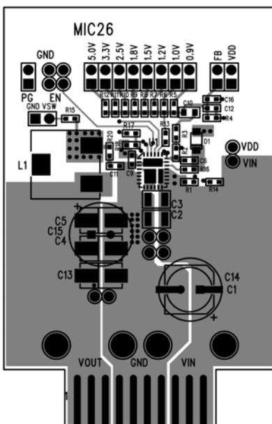
Figure 9. MIC26901 Evaluation Board Top Layer
