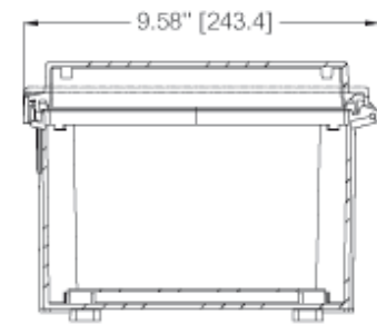
Hinged screw cover
