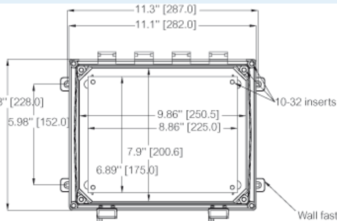
Top View - cover removed
