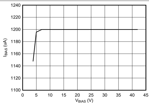
Figure 7-4. V BIAS vs I BIAS (Active Mode)
