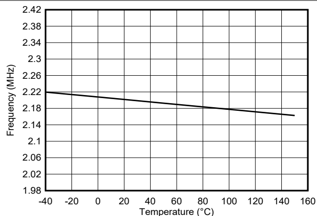
Figure 7-2. Frequency vs Temperature (RT = 9.09 kΩ, 2.2 MHz)
