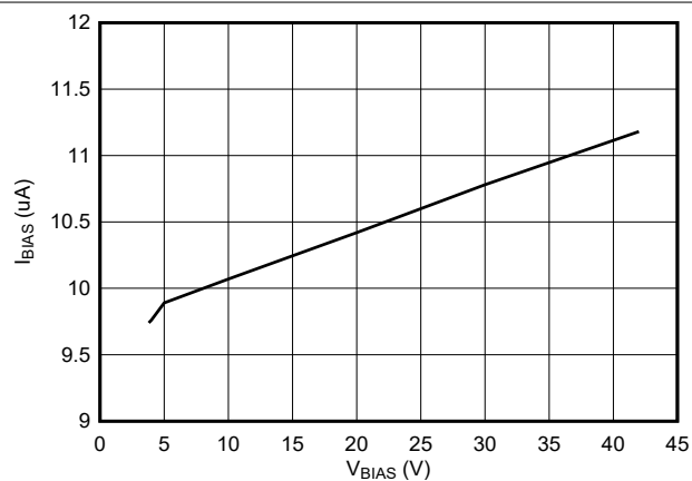
Figure 7-6. V BIAS vs I BIAS (Bypass Mode, Charge Pump Off)
