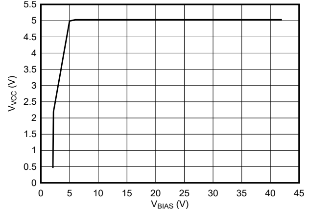
Figure 7-8. V BIAS vs V VCC
