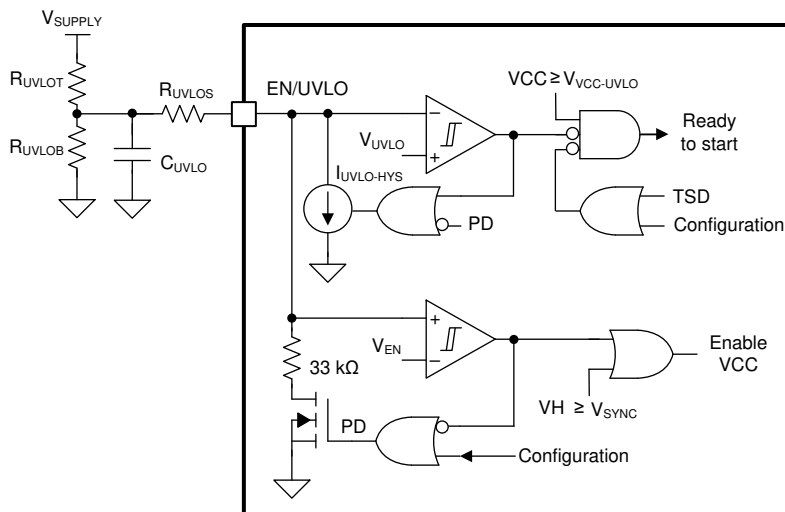
Figure 8-1. EN/UVLO Circuit
