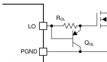
Figure 8-20. Slew Rate Control
