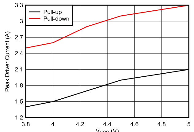
Figure 7-10. V VCC vs Peak Driver Current
