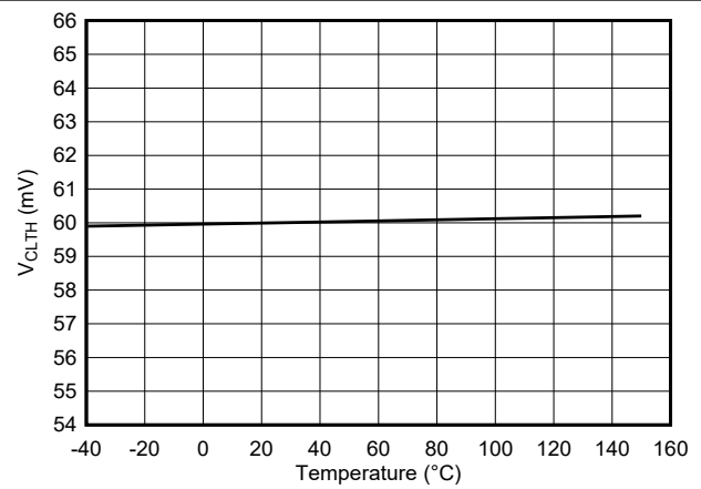
Figure 7-12. Peak Current Limit Threshold V CLTH vs Temperature (CSP = 3 V)
