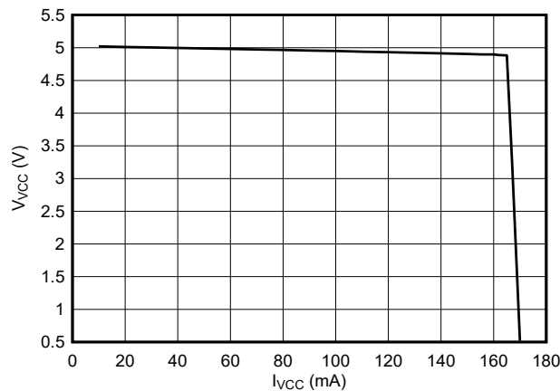
Figure 7-9. V VCC vs I VCC
