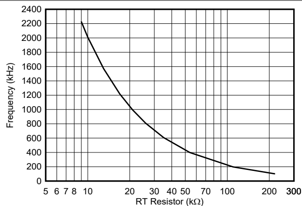
Figure 7-1. Frequency vs RT Resistance
