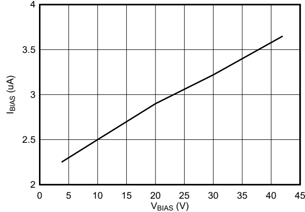
Figure 7-7. V BIAS vs I BIAS (Shutdown Mode)
