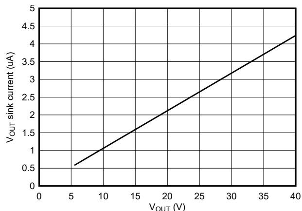
Figure 7-14. V_{OUT} Sink Current vs V_{OUT} (Deep Sleep)
