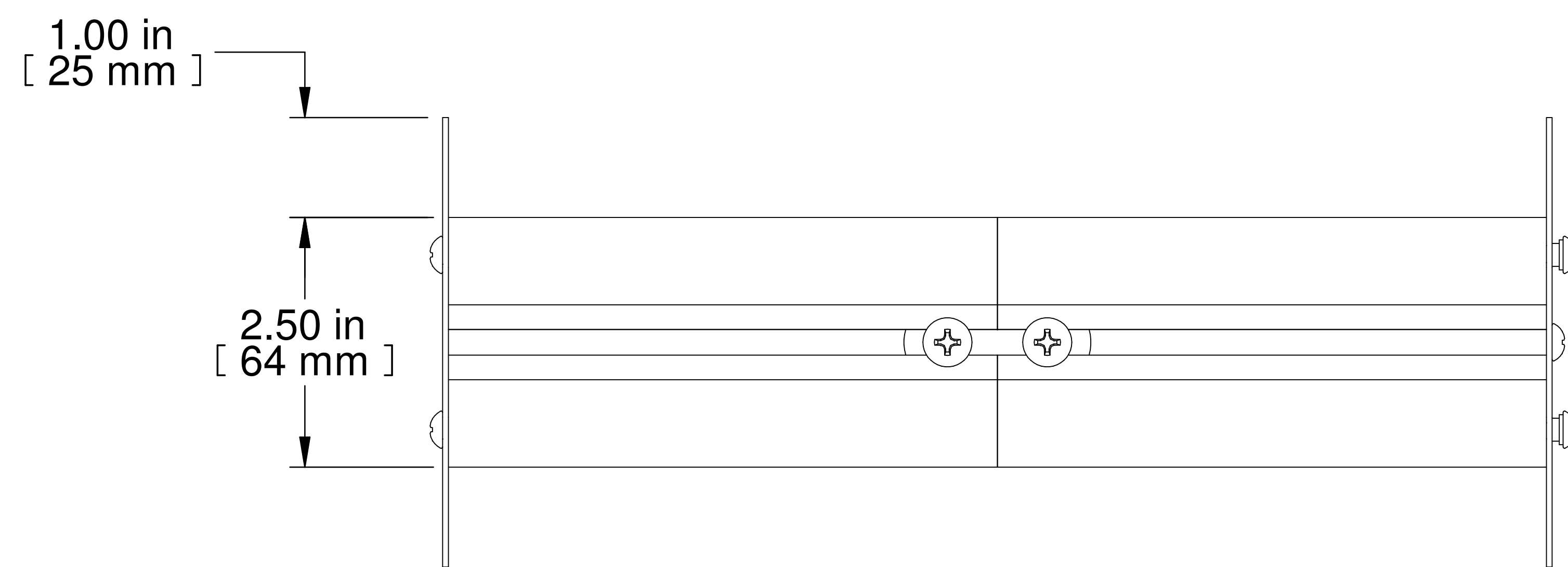
R.S. VIEW
