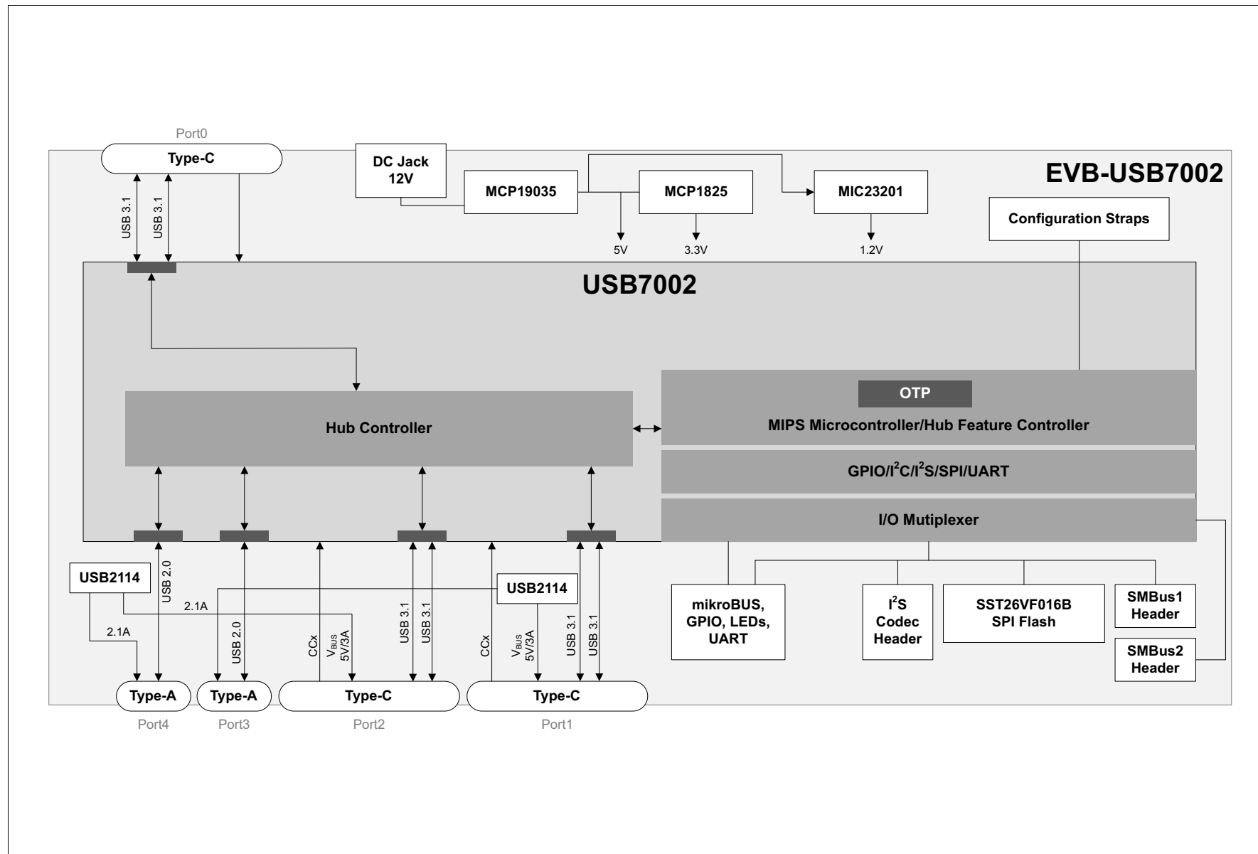
FIGURE 1-1: EVB-USB7002 BLOCK DIAGRAM
