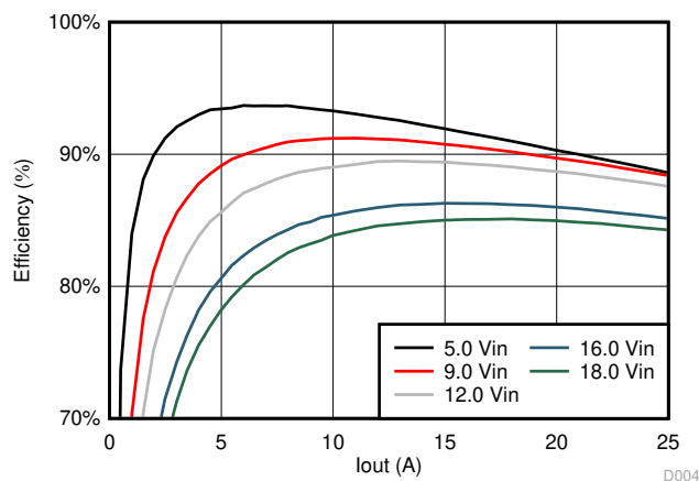
Figure 9-1. Efficiency of 0.9-V Output vs Load
