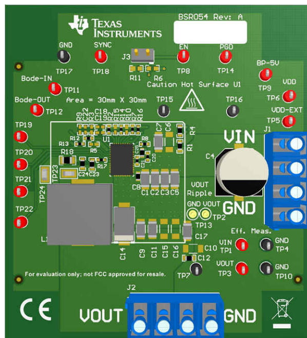
Figure 6-1. BSR054EVM Overview
