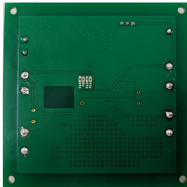
Figure 2. BD9F500QUZ-EVK-001 (Bottom View)
