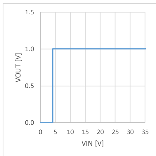
Figure 10. Line Regulation ( I_o = 0\text{mA} )
