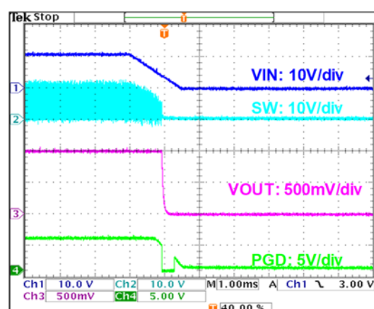
Figure 17. Shutdown Waveform ( I_O = 1A )
