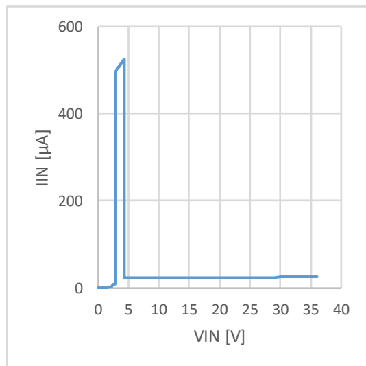
Figure 8. Current Consumption vs VIN ( I_o = 0\text{mA} )
