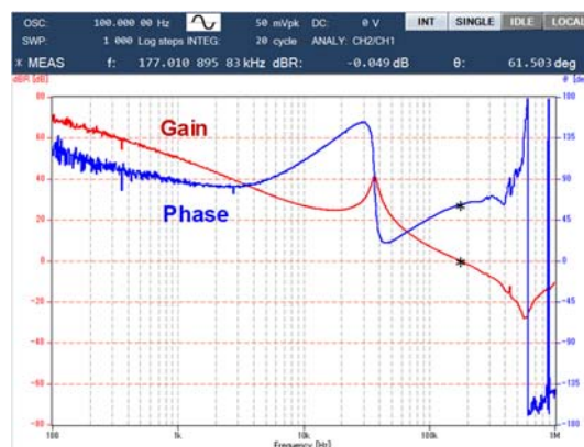
Figure 15. Frequency Response ( I_O = 5A )
