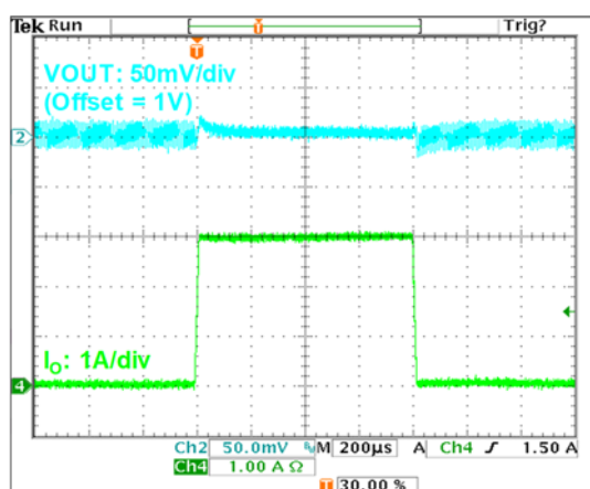
Figure 14. Load Response
