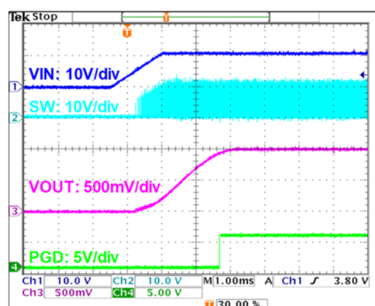
Figure 16. Start Up Waveform ( I_O = 1A )
