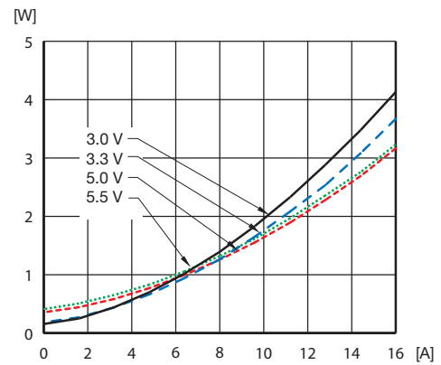
Dissipated power vs. load current and input voltage at T_{ref} = +25\text{ °C}
