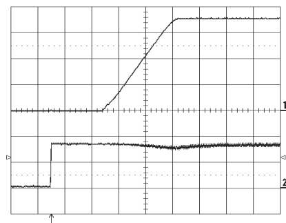
Start-up at I_O = 16\text{ A} resistive load at T_{ref} = +25\text{ °C} , V_{in} = 3.3\text{ V} . Start enabled by connecting V_{in} . Top trace: output voltage (0.5 V/div.). Bottom trace: input voltage (2 V/div.). Time scale: 2 ms/div.
