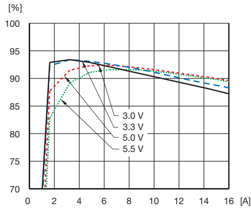
Efficiency vs. load current and input voltage at T_{ref} = +25\text{ °C}
