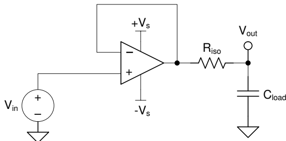
Figure 7-5. Extending Capacitive Load Drive With the TLV9151-Q1
