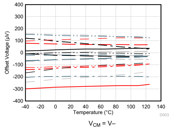
Figure 6-4. Offset Voltage vs Temperature
