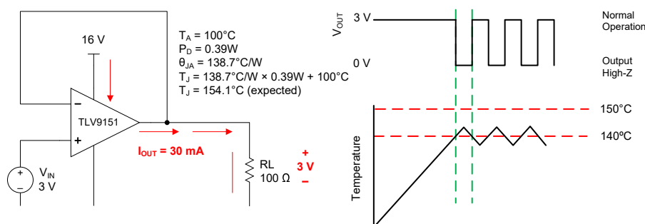
Figure 7-2. Thermal Protection
