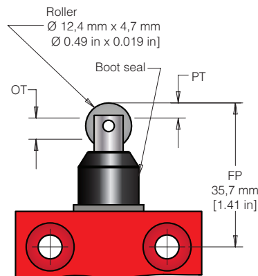
Figure 10. 24CE31 Dimensions
